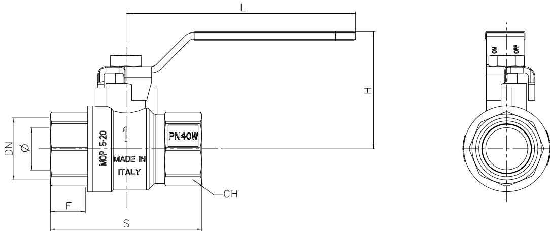
Dimensions (mm)
